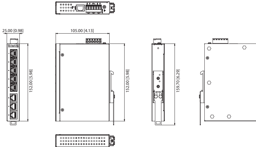
Panel Cut-out Dimensions (W x H x D): 25 x 152 x 105 mm (0.98 x 5.98 x 4.13 inch)
